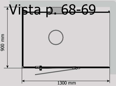
VISTA 130 LEFT Size: D 900 x W 1300 mm
