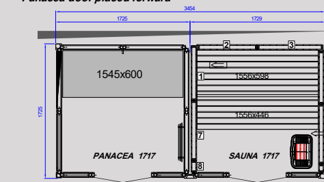
Alt. 1 - Placed in right corner, Panacea door placed forward
