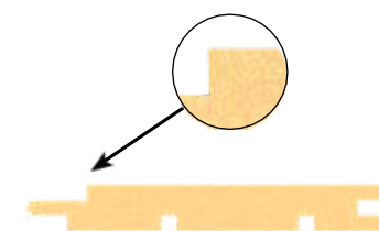
2. SAUNA PANEL STS PROFILE
