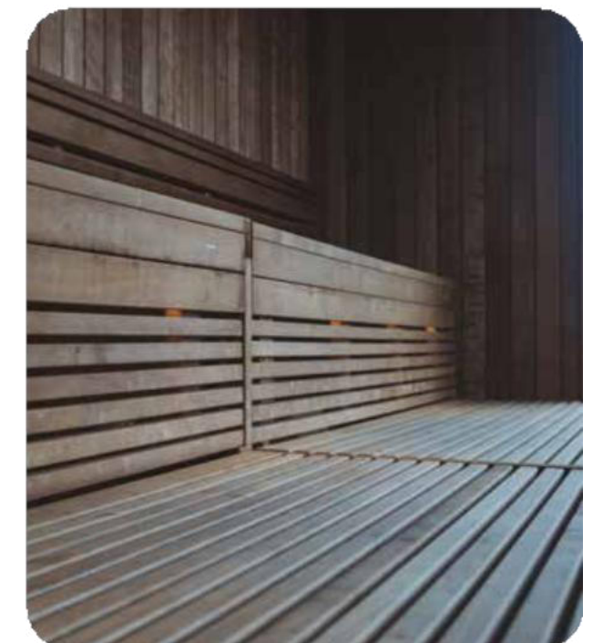
SKIRTING PANELS Prefabricated skirting panels screen off the gaps between the benches.
