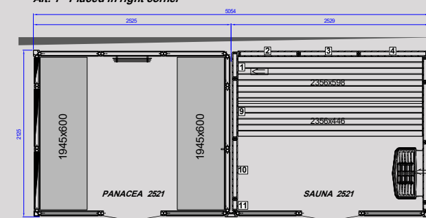
TWIN PANACEA 2521 Size: D 2125 x W 5054 mm
